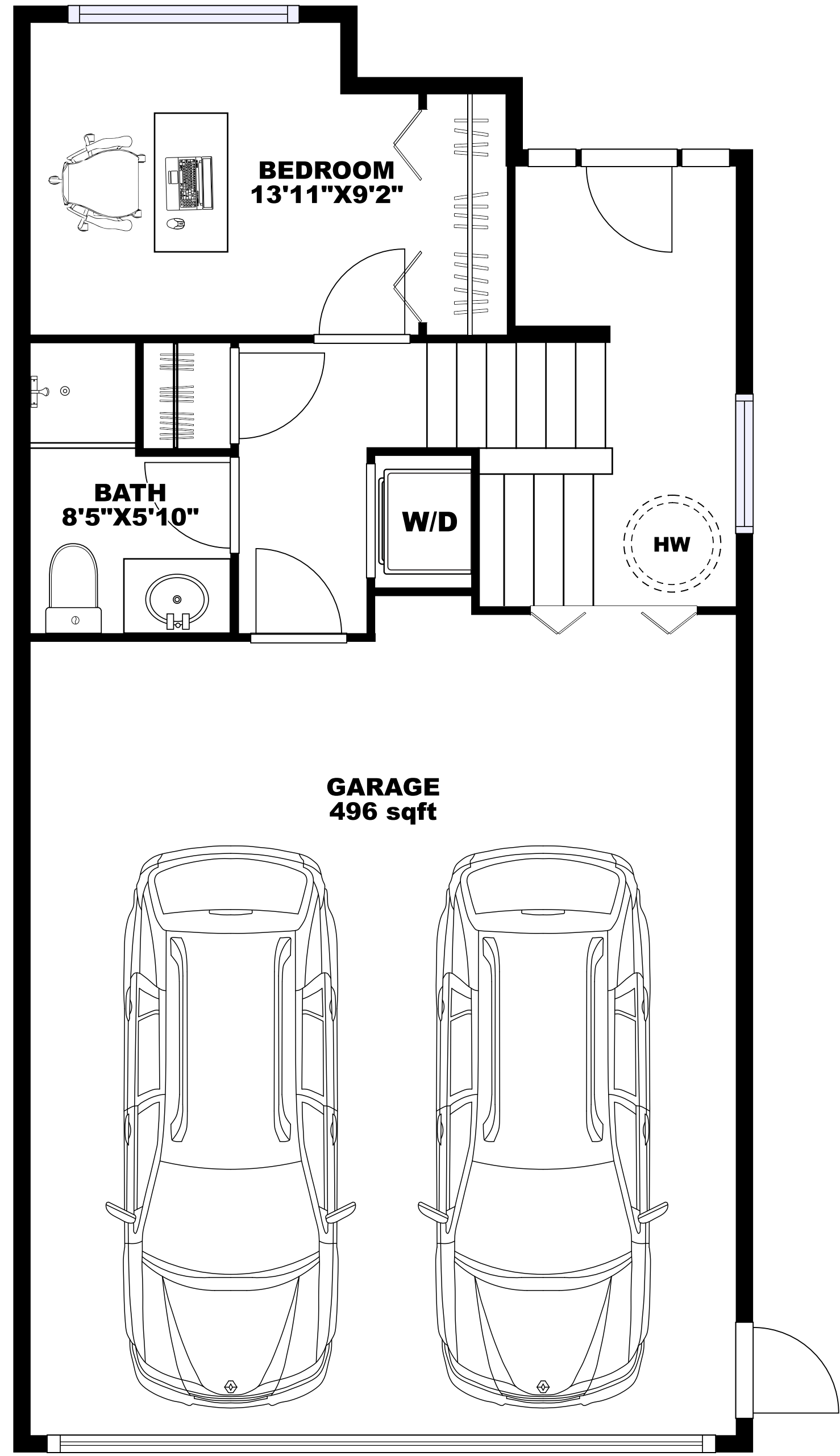
BASEMENT
