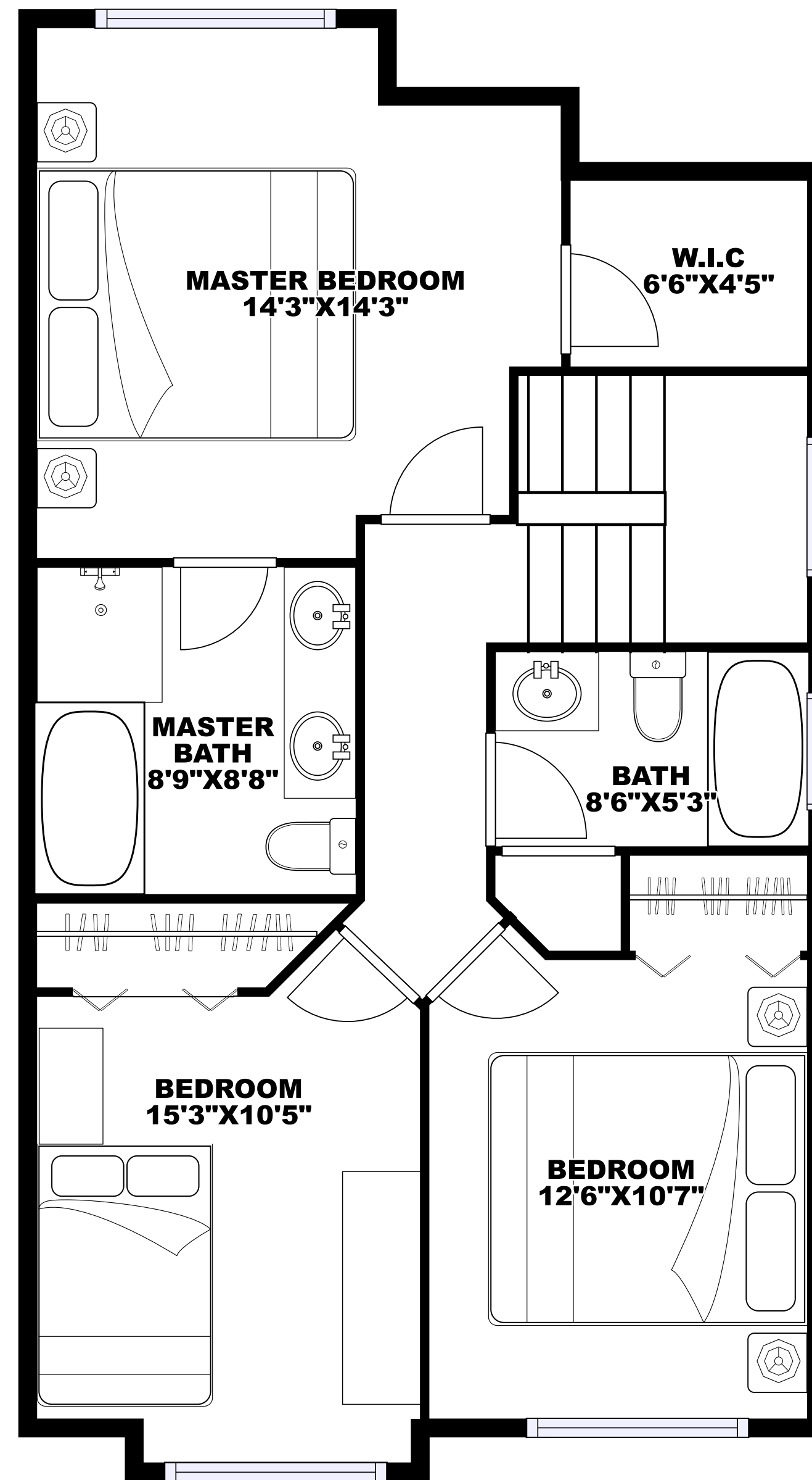
UPPER FLOOR
